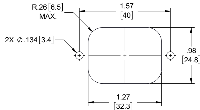
FIXING DETAILS
