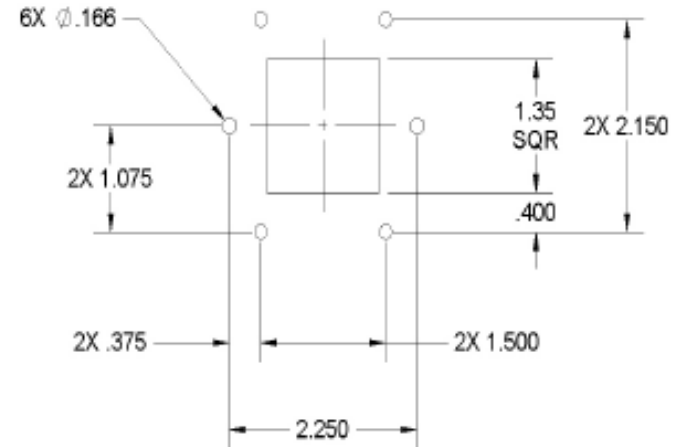
Figure 1 Recommended Panel Thickness: 10 through 22 gauge steel (0.135 to 0.030)
