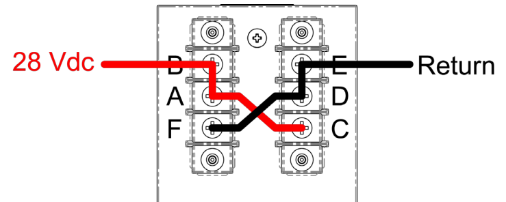
Figure 2 Wiring Diagram for 30A Applications
